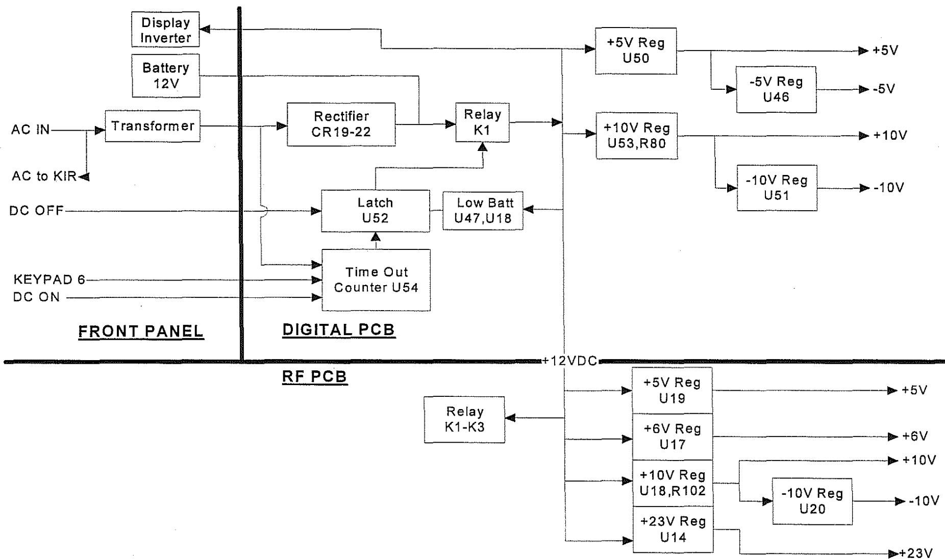
T-48D Power Distribution Function Flow Figure 3-1
