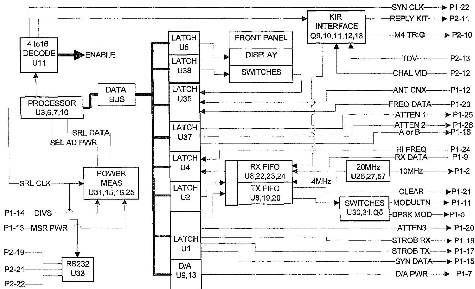
T-48D Digital PCB Function Flow Figure 3-2
