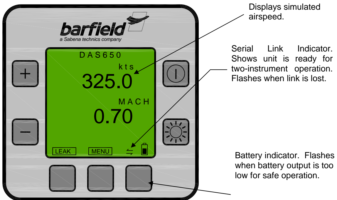
FIGURE 2 AERONAUTICAL DISPLAY
